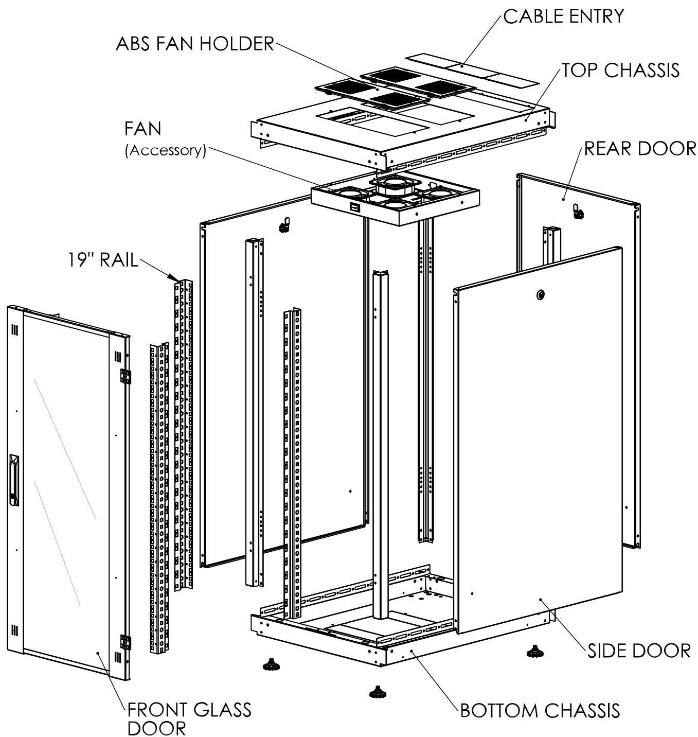
Exploded view
