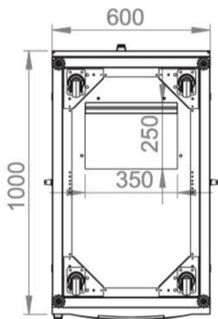
Bottom view
